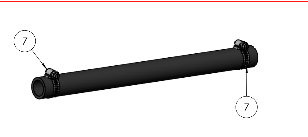
2 COMPLETE INLET HOSE [CUT LENGTH] 890mm 3/4"
