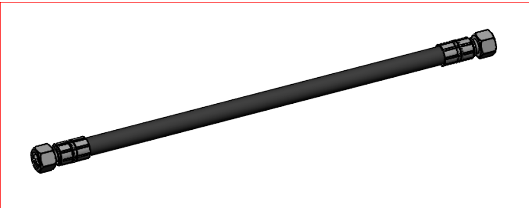
2 COMPLETE INLET HOSE [CUT LENGTH] 890mm 3/4"
