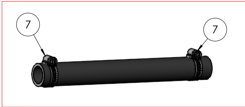
5 COMPLETE WATER TANK INLET HOSE [CUT LENGTH] 255mm 1"
