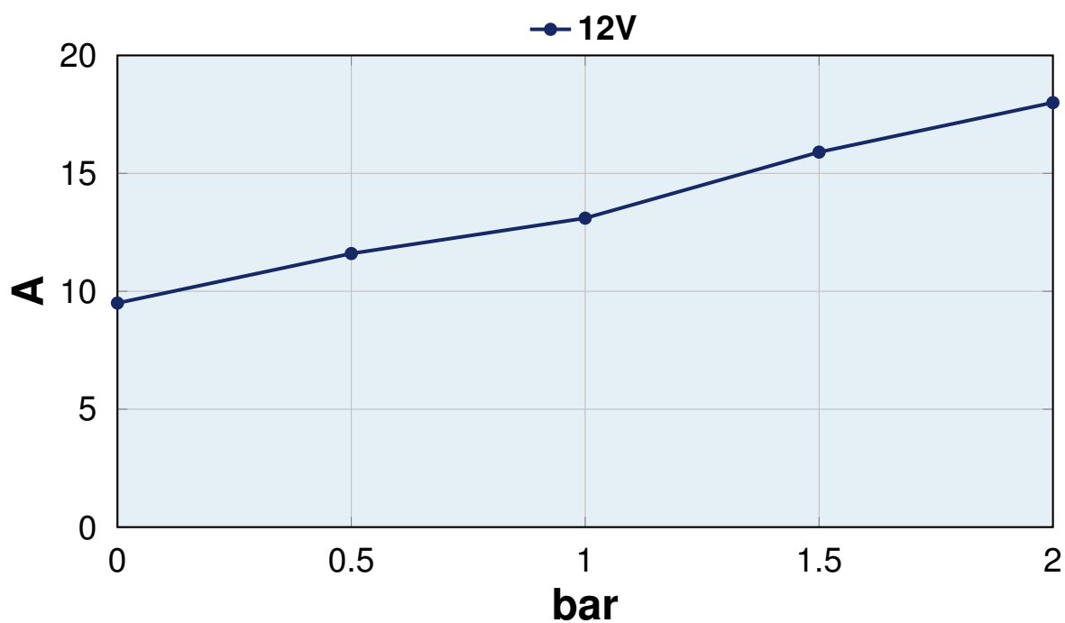
AMPERE-DRAW DIAGRAM
