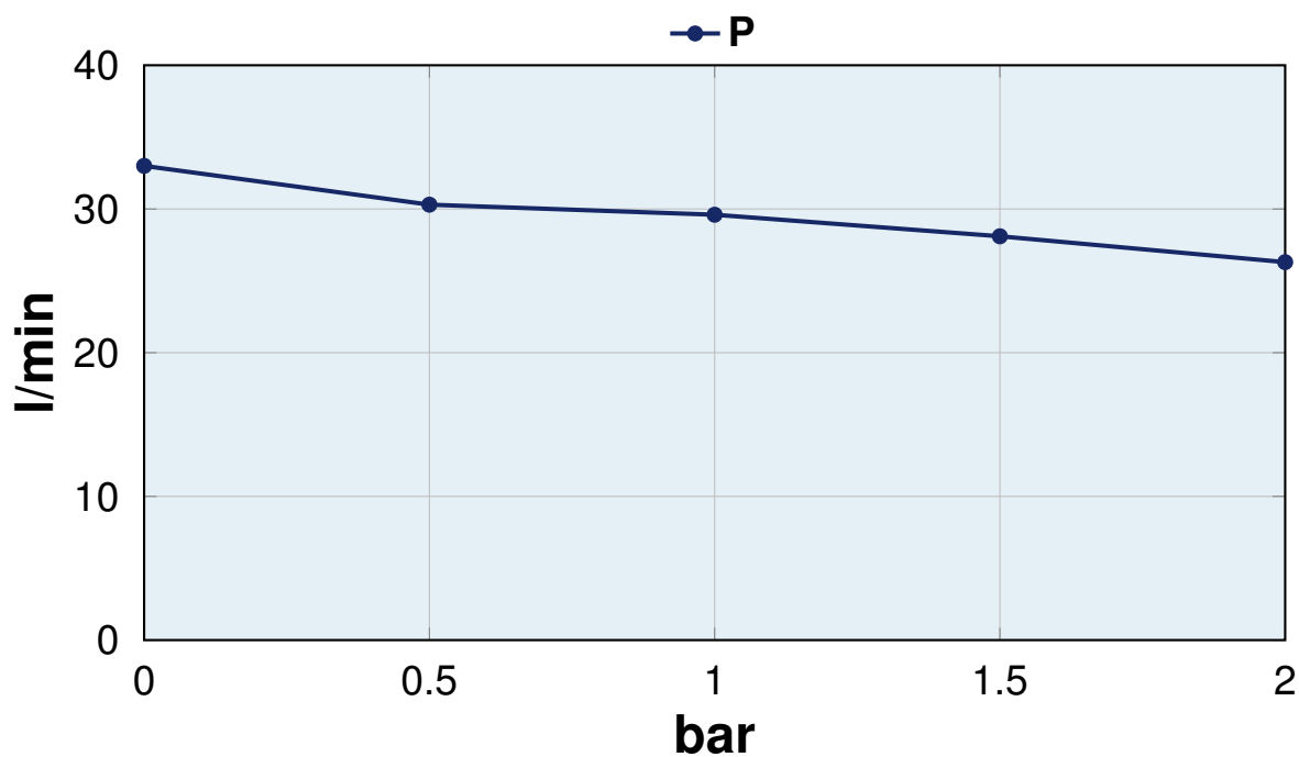
FLOW RATE DIAGRAM
