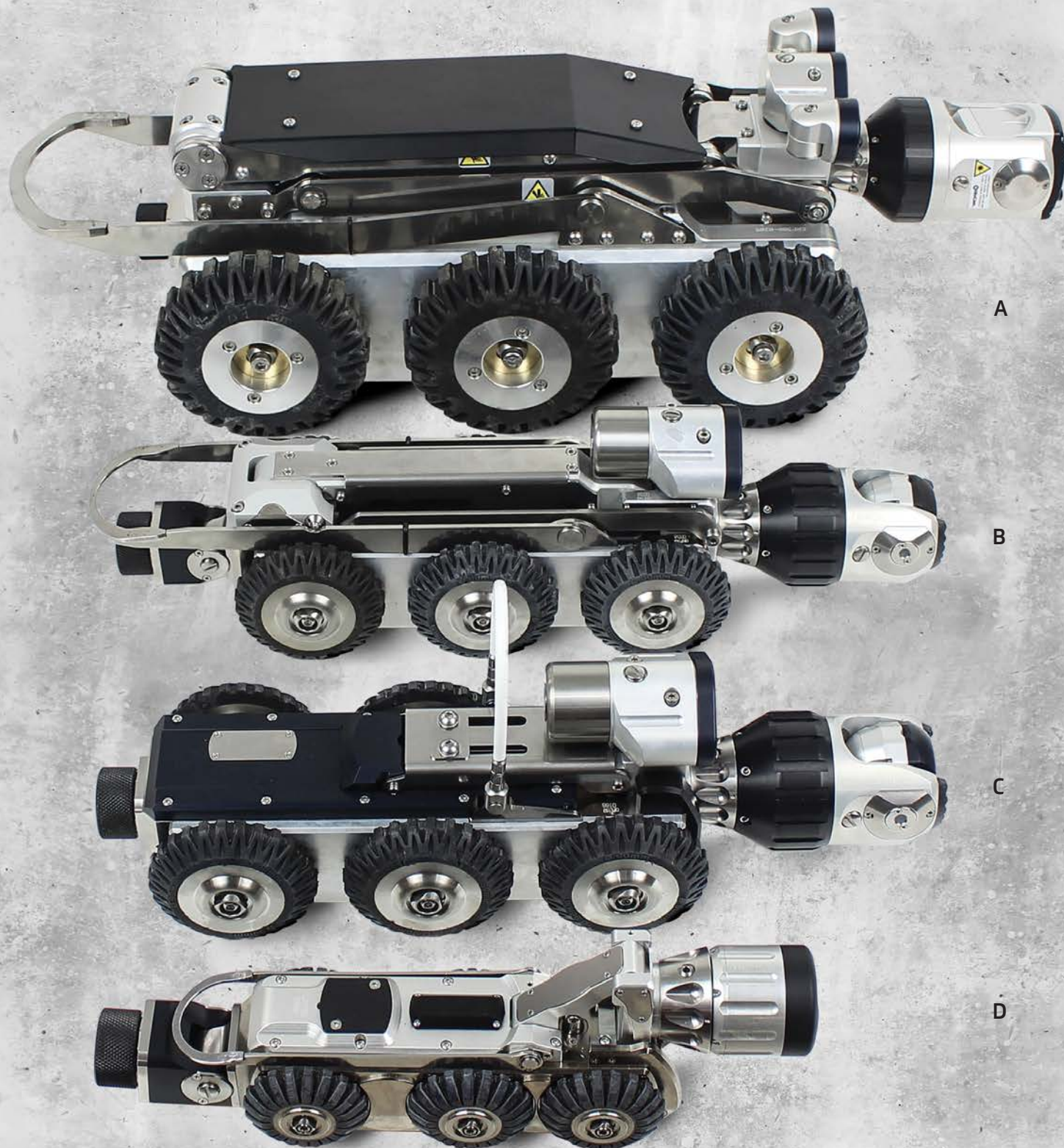
A - CRP300 Crawler, CAM028L Pan, Rotate, Zoom & Laser, ALN300 Auxiliary Lights B - CRP140 Crawler, CAM028 Pan & Rotate, ALB300 Auxiliary Light/Backeye C - CPL150S Crawler, CAM026 Pan & Rotate, ALB300 Auxiliary Light/Backeye D - CRP90 Crawler, CAM027 Axial
